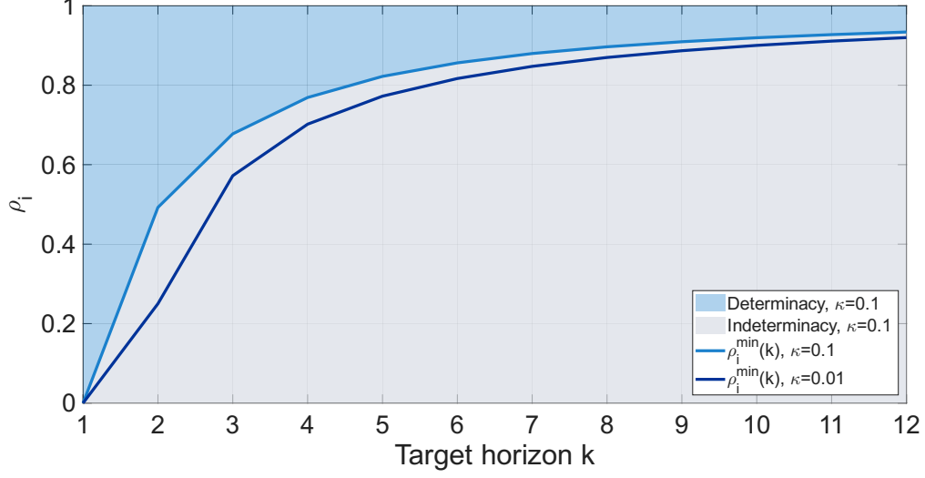
Figure 7: Determinacy region as a function of target horizon k and interest rate smoothing \rho_i for \beta = 0.99, \phi_\pi = 1.5 .
