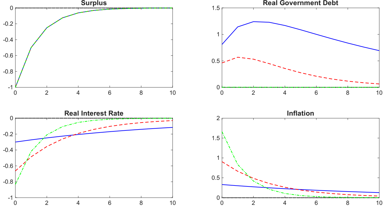
Figure 3: Impulse response functions after negative surplus shock of unity for k = 3 , \beta = 0.99 , \phi_\pi = 0 , \alpha_b = 0 , \alpha_y = 0 , \rho_g = 0.5 , \gamma = 0.6 , with \kappa = 0.1 (blue, solid lines), \kappa = 0.5 (red, dashed lines), \kappa = 0.01 (green, dash-dotted lines).
