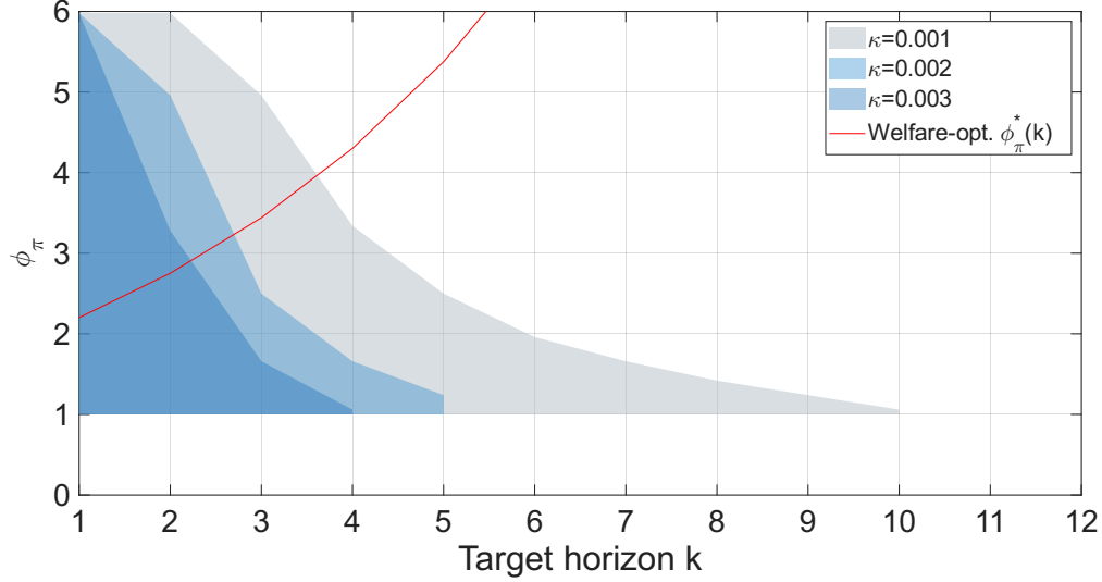
Figure 2: Determinacy region as a function of target horizon k and policy parameter \phi_\pi for different values of \kappa with \beta = 0.99 and the welfare maximizing \phi_\pi^*(k) .
