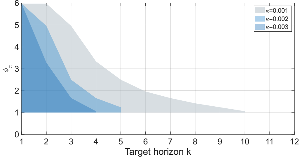
Figure 1: Determinacy region as a function of target horizon k and policy parameter \phi_\pi for different values of \kappa with \beta = 0.99 , based on the model of Section 4.
