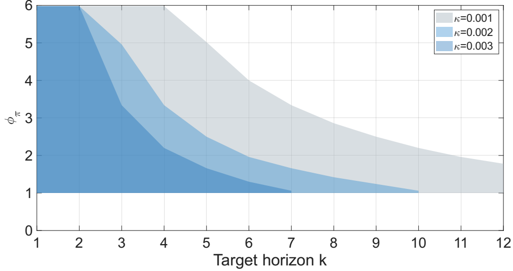
Figure 8: Determinacy region as a function of target horizon k and policy parameter \phi_\pi for different values of \kappa with \beta = 0.99 .
