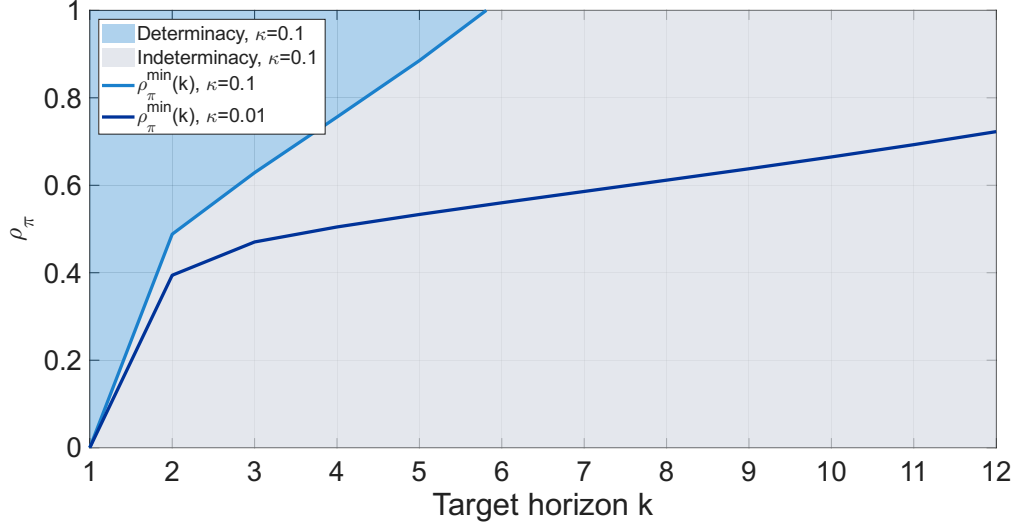
Figure 5: Determinacy as a function of target horizon k and inflation inertia \rho_\pi for \beta = 0.99, \phi_\pi = 1.5 .
