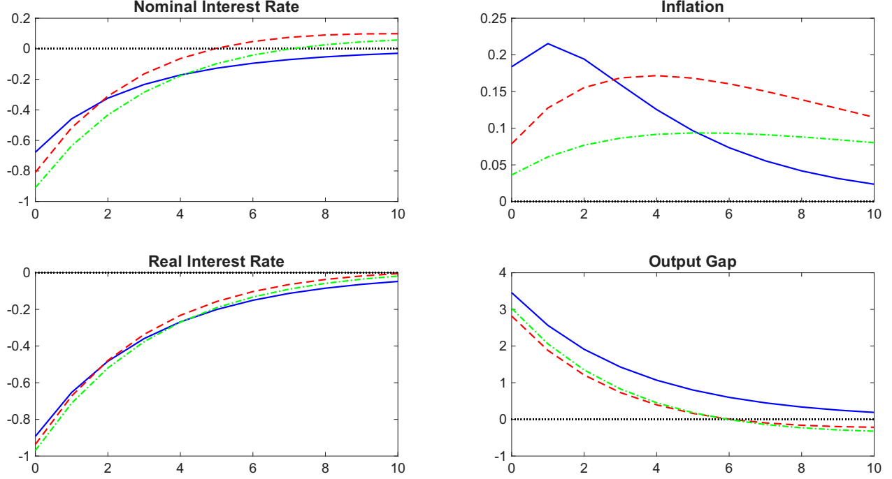
Figure 4: Impulse response functions after contractionary monetary policy shock of unity for k=1 , \beta=0.99 , \kappa=0.1 , \phi_\pi=1.5 , \rho_\nu=0.75 , \gamma=0 , with \rho_\pi=0.3 (blue, solid lines), \rho_\pi=0.6 (red, dashed lines), \rho_\pi=0.9 (green, dash-dotted lines).
