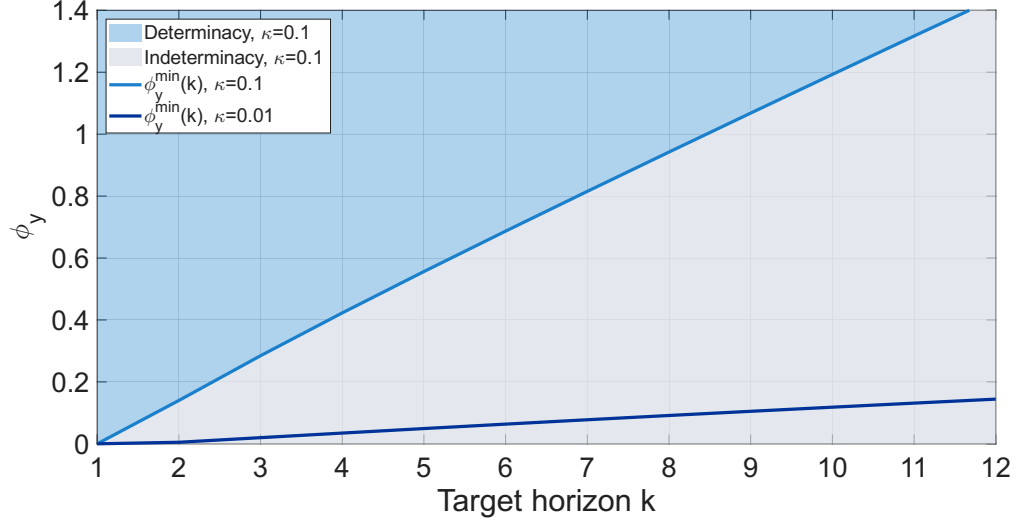
Figure 6: Determinacy region as a function of target horizon k and output-gap coefficient \phi_y for \beta = 0.99, \phi_\pi = 1.5 .
